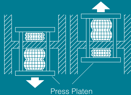
FORMING PRESS
